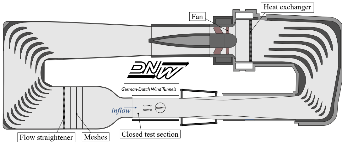
Figure 18: Schematic of low-speed wind tunnel DNW-NWB.
