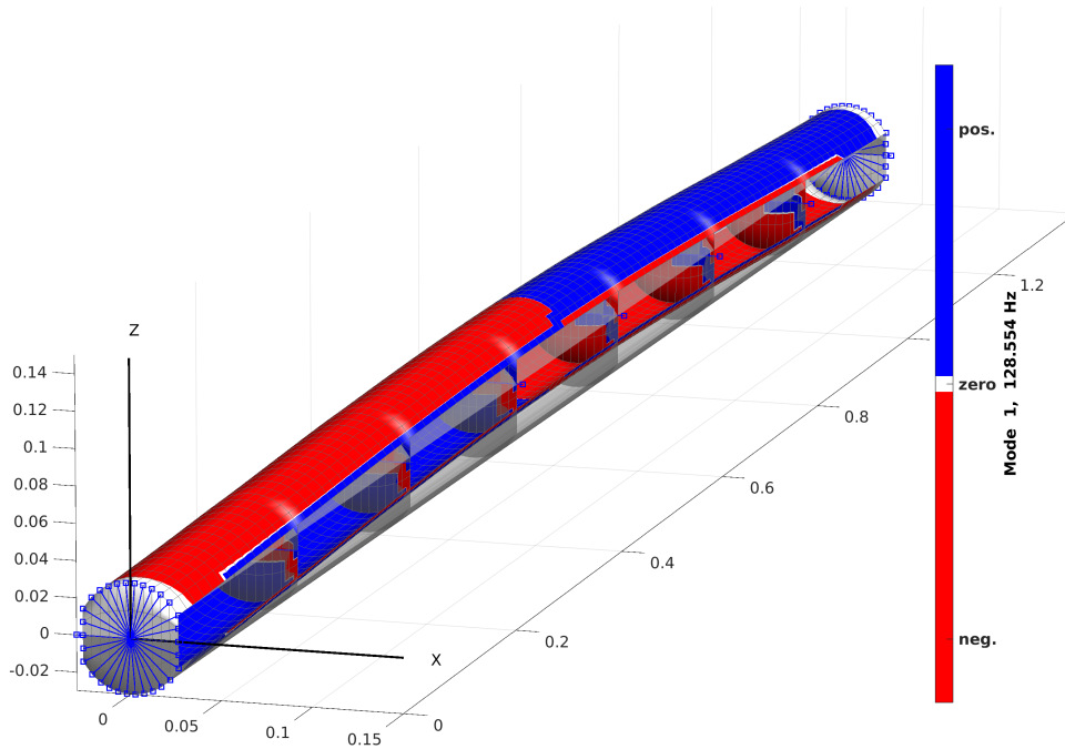
Figure 17: Illustration of the RSC's first eigenmode (here corresponding to its first bending mode).
