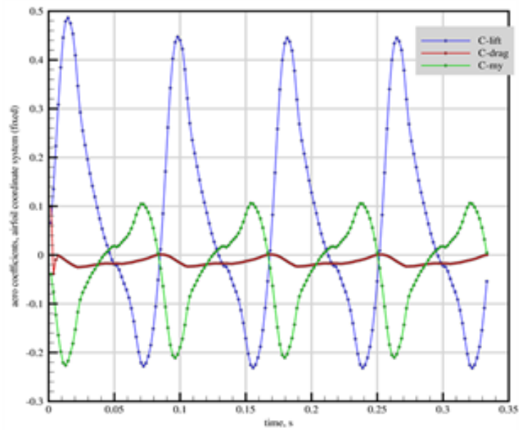
Figure 4: Aerodynamic loads generated by the stationary airfoil.
